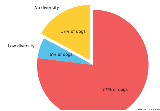
MHC Class II - DLA DQA1 and DQB1 No Diversity
