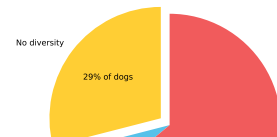
MHC Class II - DLA DQA1 and DQB1 No Diversity
