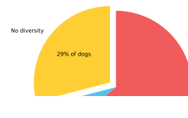
MHC Class II - DLA DQA1 and DQB1 No Diversity
